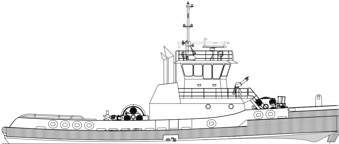
OUTBOARD PROFILE
