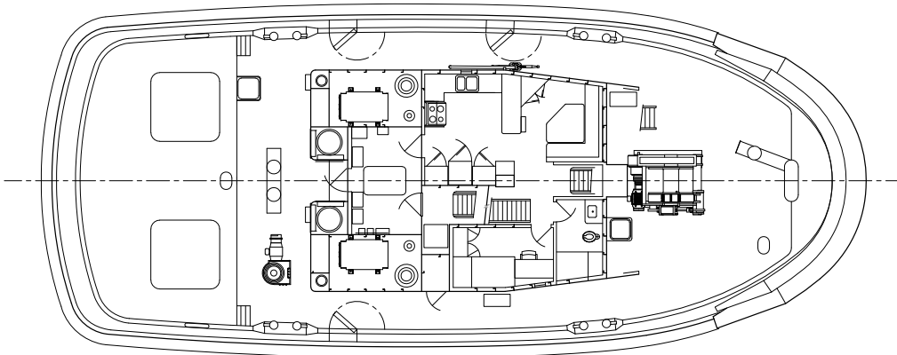
MAIN DECK
