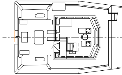
BRIDGE DECK
