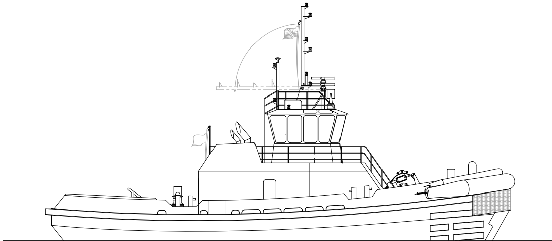
OUTBOARD PROFILE
