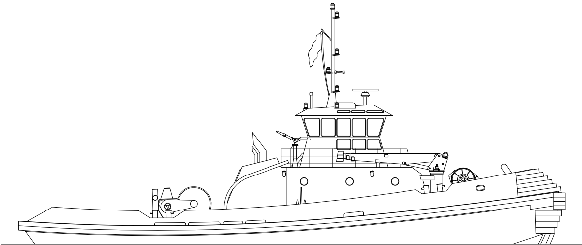
OUTBOARD PROFILE
