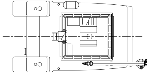
BRIDGE DECK
