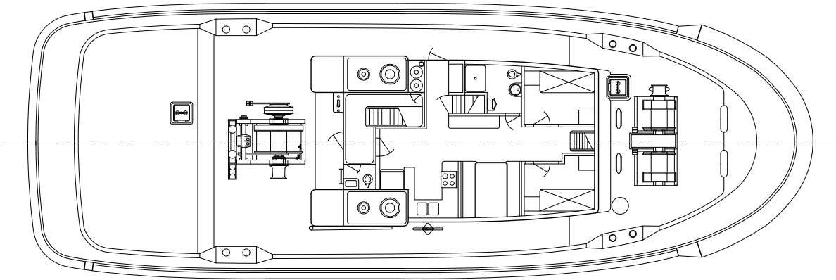
MAIN DECK
