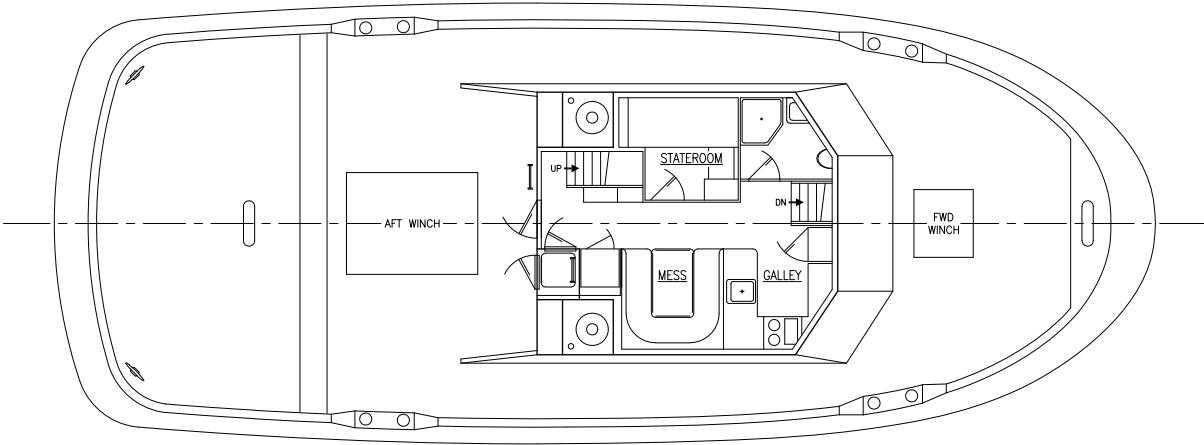
MAIN DECK
