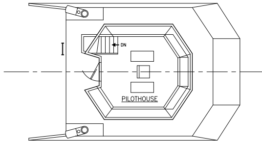
BRIDGE DECK
