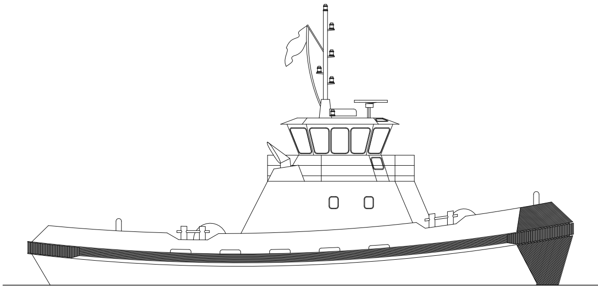
OUTBOARD PROFILE
