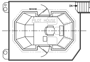
BRIDGE DECK
