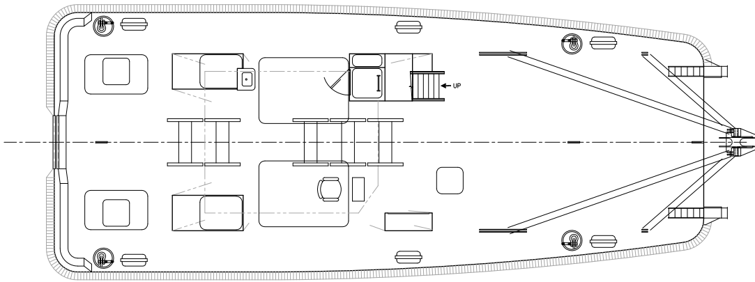
MAIN DECK
