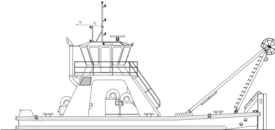
OUTBOARD PROFILE
