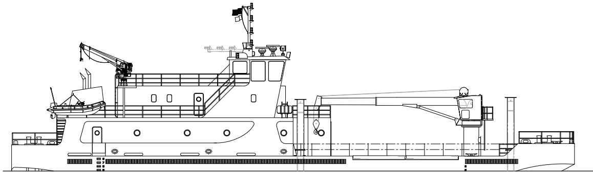
OUTBOARD PROFILE
