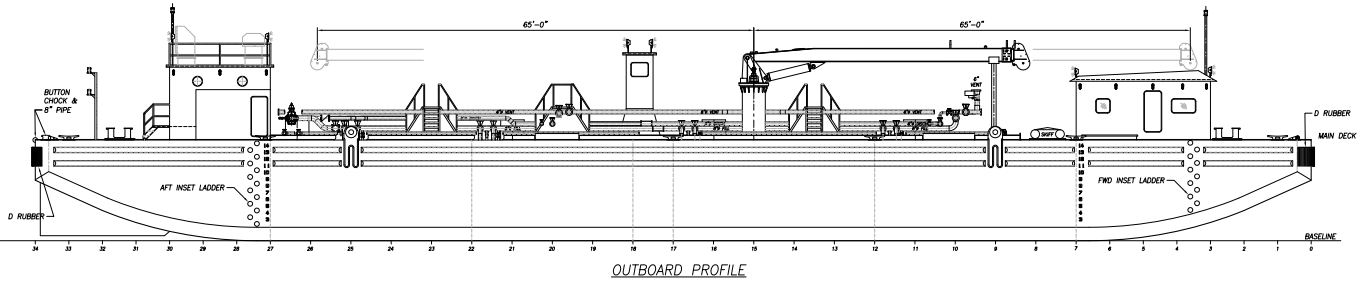
OUTBOARD PROFILE
