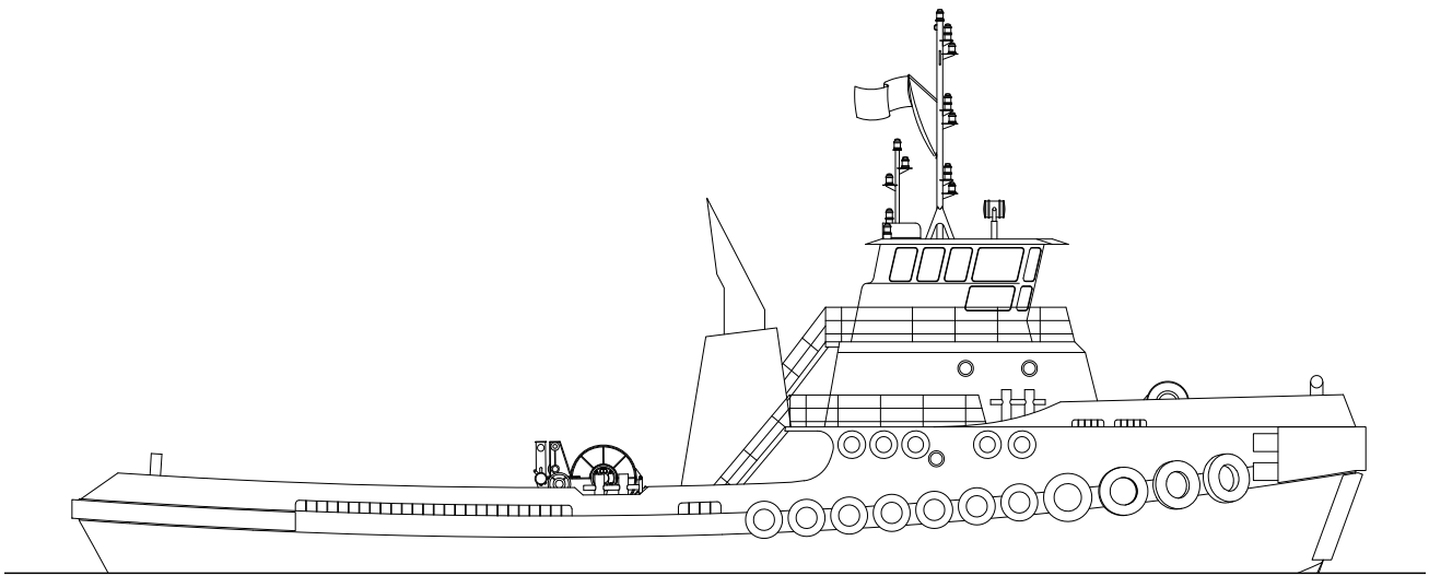
OUTBOARD PROFILE
