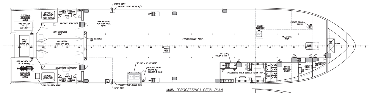
MAIN (PROCESSING) DECK PLAN
