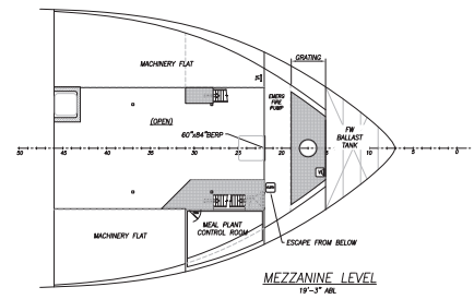
MEZZANINE LEVEL 17'-3" ABL
