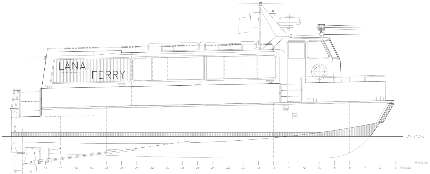
OUTBOARD PROFILE
